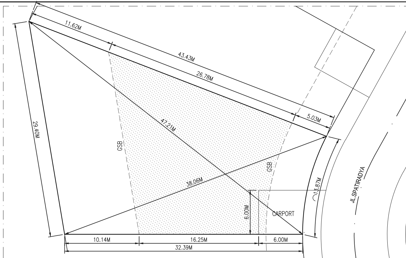
DENAH UNIT HUNIAN JL.SPATIRADYA NO. 18 SKALA 1 : 300
