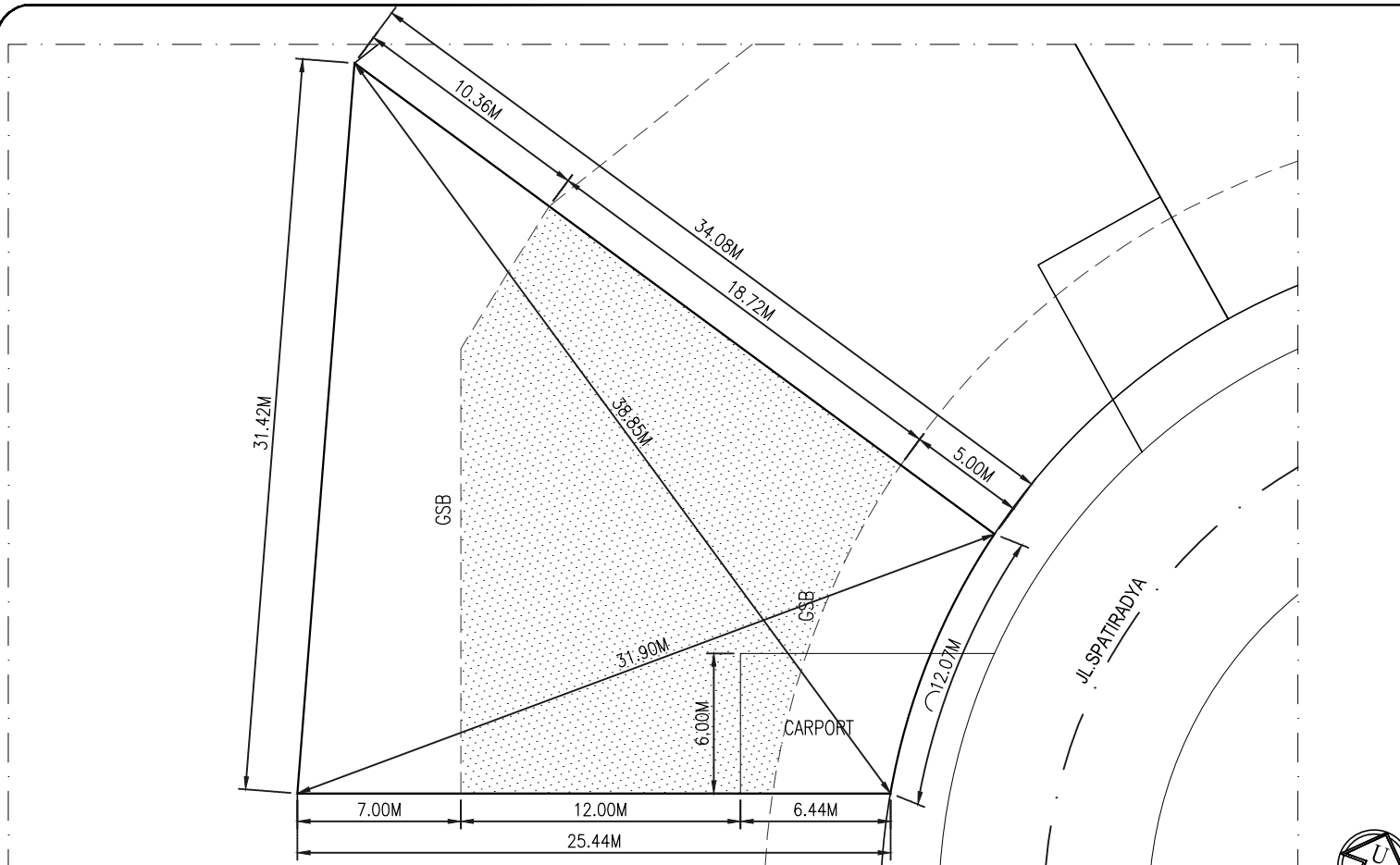
DENAH UNIT HUNIAN JL.SPATIRADYA NO. 22 SKALA 1 : 300
